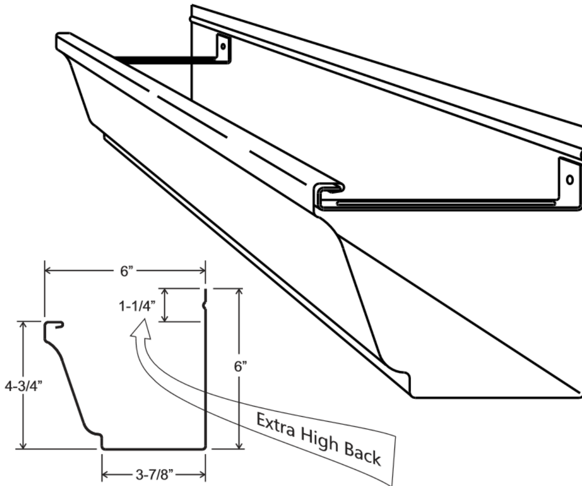
Gutter Profile
