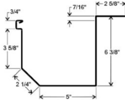
Flanged Back Profile
