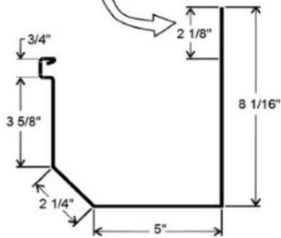
Straight Back Profile
