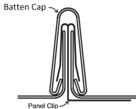
Seam Profile
