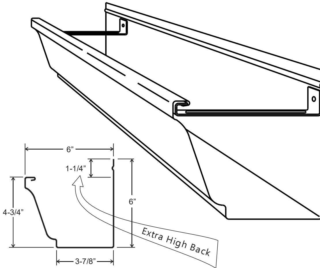
Gutter Profile
