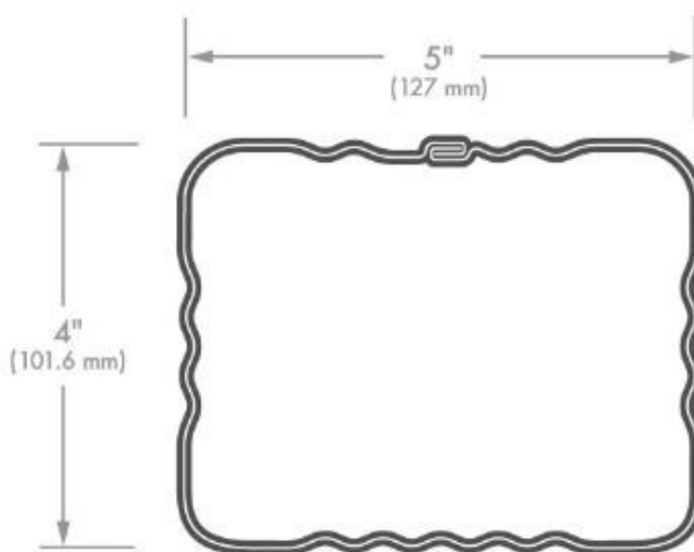
4X5 CORRUGATED A ELBOW
