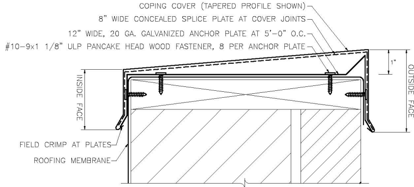
MOC2 COPING SYSTEM - TAPERED
